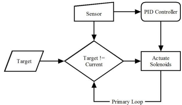
Figure 5: Primary Control Theory
