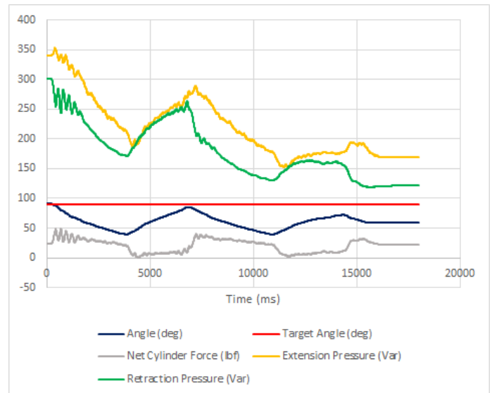
Figure 10: Force Control Compensation with User Controlled Motion (51bm Load)
