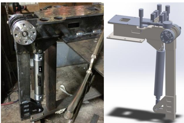
1 - Pneumatic Cylinder
