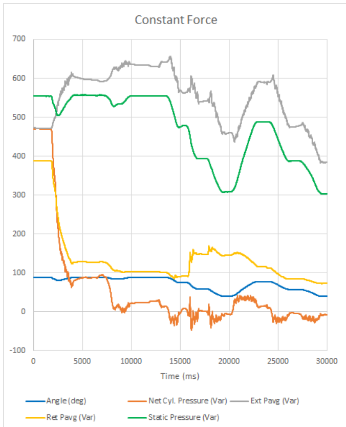
Figure 13: Force Compensation with User Controlled Motion, 40lbm end load
