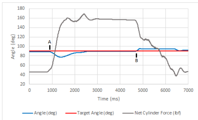
Figure 9: Effects of Impulse on the Static Apparatus
